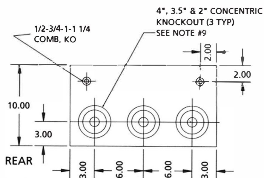
BOTTOM VIEW
