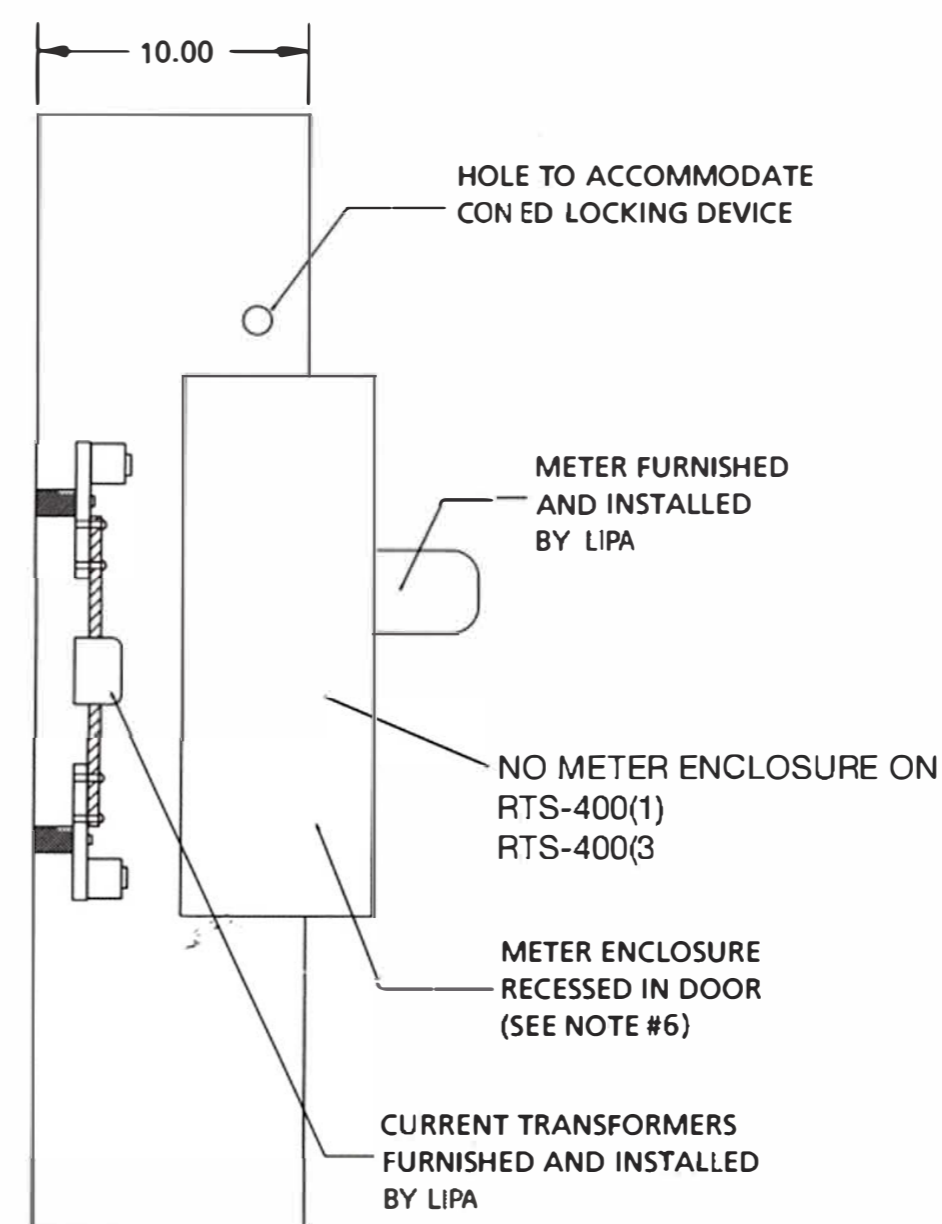
SIDE VIEW
