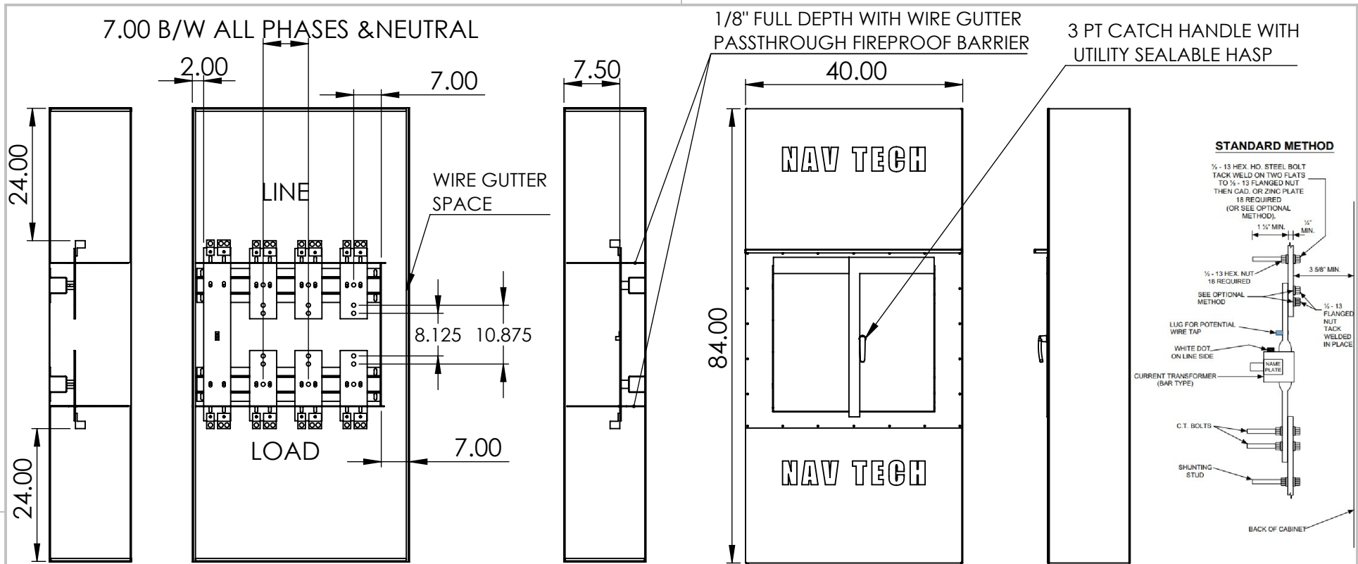
PHASE SIDE VIEW OPEN FRONT VIEW NEUTRAL SIDE VIEW COVERED FRONT VIEW COVERED SIDE VIEW CT INSTALLED VIEW
