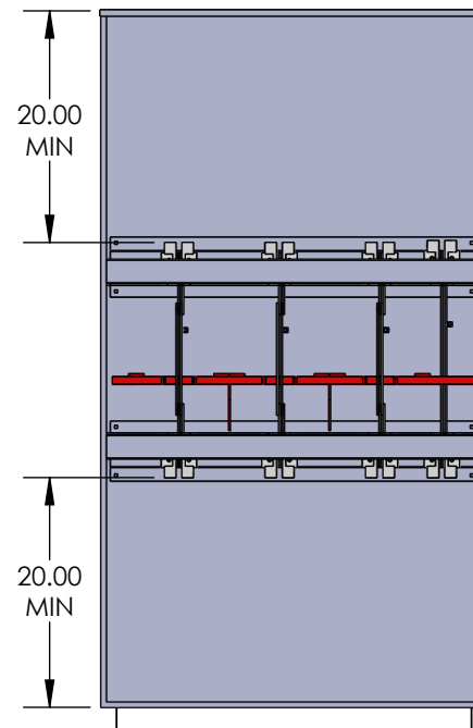
OPENED FRONT VIEW
