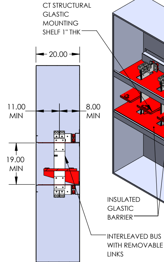
SECTIONED SIDE VIEW
